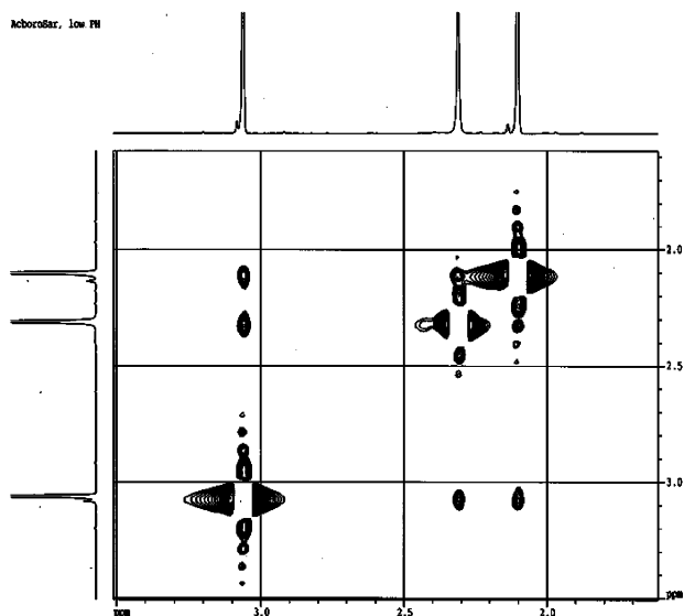
FIGURE 3. (A) Stack plot of 1D ^1\text{H} 300 MHz NMR spectra of 2b in 90% \text{H}_2\text{O} /10% \text{D}_2\text{O} at 25 ^\circ\text{C} and various values of the pH. Forms A , B , and C are described in the text; decomposition products are indicated with an asterisk. (B) 2D ^1\text{H}/^1\text{H} NOESY spectrum of 2b at pH \sim 2 . The NOE peaks between H-b and H-c indicate a trans conformer.
