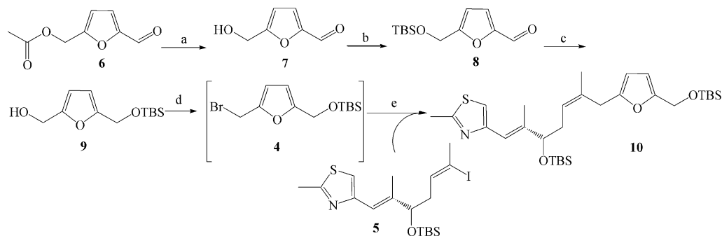
Scheme 2. Synthesis of the C7–C12 fragment 4 and Pd-mediated coupling of building blocks 4 and 5 . a) \text{K}_2\text{CO}_3 (0.16 equiv), \text{CH}_3\text{OH} , RT, 18 h, 98 %; b) TBSCl (1.2 equiv), imidazole (1.8 equiv), DMF, RT, 18 h, 89 %; c) \text{NaBH}(\text{OAc})_3 , benzene, reflux, 3 h, 93 %; d) \text{PPh}_3 (1.1 equiv), imidazole (1.2 equiv), \text{Br}_2 (1.1 equiv), \text{CH}_2\text{Cl}_2 , 0 °C, 10 min, complete by TLC; e) \text{Zn}^* (6.0 equiv) in THF, –30 °C; then 4 in THF added by syringe pump over 4.5 h, [\text{Pd}(\text{PPh}_3)_4] (12.5 mol %); then 5 in THF, 60 °C, 1 h, 85 %.
