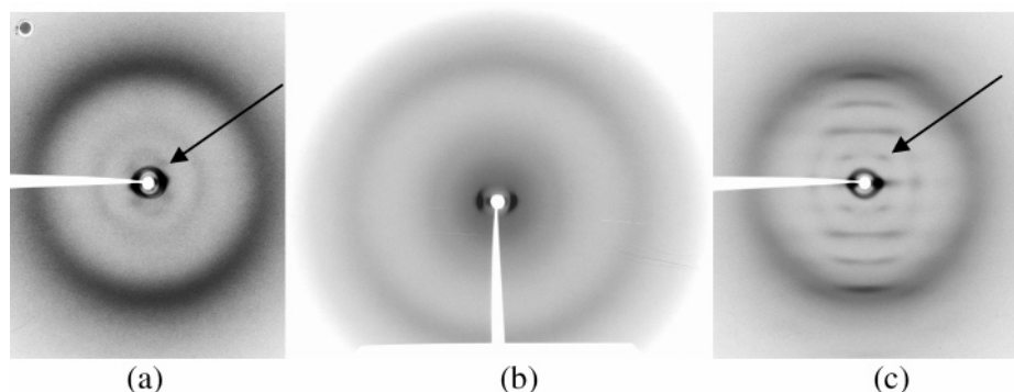
Figure 5. X-ray pattern of an aligned sample in the Col h mesophase: (a) compound 8 taken at room temperature; (b) compound 9 taken at 40 °C; (c) compound 11 taken at room temperature. The capillary axis is vertical. Diffuse spots in the first layer line are indicated with an arrow.
