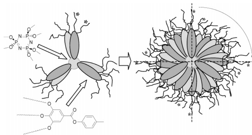
Figure 6. Schematic model for the helical columnar assembly of cyclotriphosphazene 11 . Four molecules rotated by 90° are needed to complete a full turn (chiral terminal chains are indicated with asterisks).
