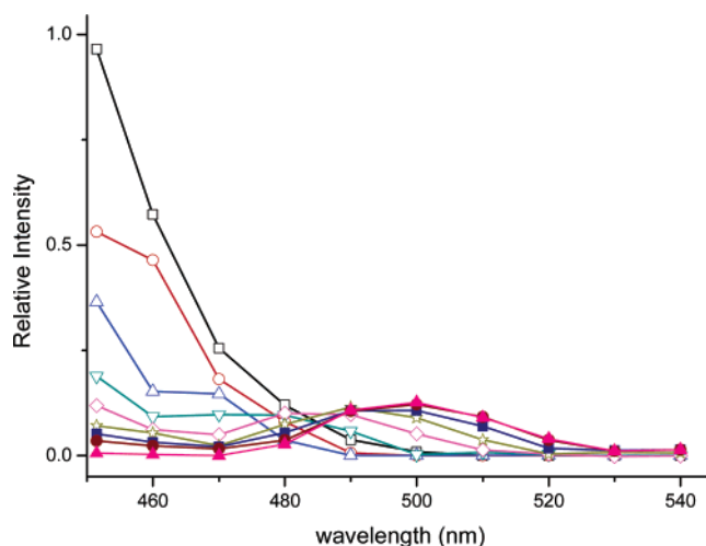
FIGURE 5. The temporal spectral evolution of D2A1 in benzene acquired at a delay time of (□) 250 fs, (○) 500 fs, (△) 1 ps, (▽) 1.5 ps, (◇) 2 ps, (☆) 3 ps, (■) 5 ps, (●) 9 ps, and (▲) 15 ps.
