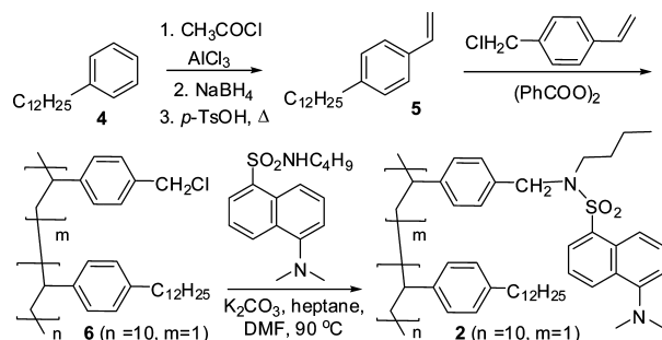
Scheme 1. Synthesis of Dansyl-Labeled Poly(4-dodecylstyrene) 2
