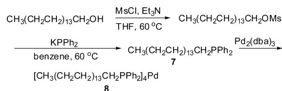
Scheme 2. Synthesis of a Polyethylene-Bound Pd(0) Catalyst
