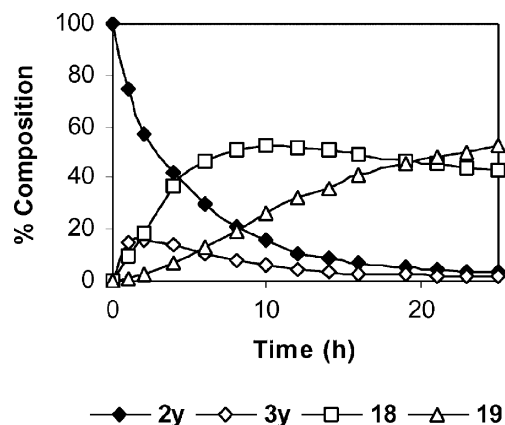
Fig. 1 The photodeconjugation reaction of dimethyl (Z)-cyclopentyl-2-butendioate 2y in the presence of triethylamine.
