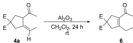
Scheme 2. Isomerisation of 4a
