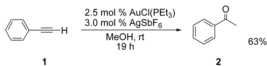
Scheme 1. Hydration of Phenylacetylene ( 1 )
