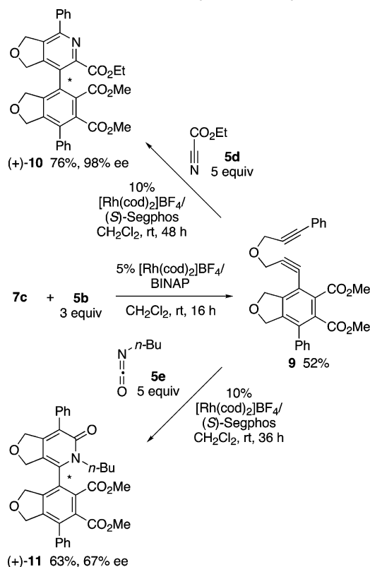
Scheme 3. Enantioselective Synthesis of Unsymmetrical Tetra- ortho -Substituted Axially Chiral Biaryls 10 and 11
