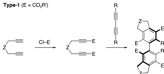
Scheme 1. Enantioselective Two-Step Synthesis of C 2 Symmetric Tetra- ortho -Substituted Axially Chiral Biaryls
