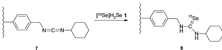
Scheme 4. Polymer-supported formation of N -cyclohexyl [\text{}^{75}\text{Se}] selenourea- N' -methyl polystyrene 8 by reaction of N -cyclohexylcarbodiimide- N' -methyl polystyrene 7 with hydrogen [\text{}^{75}\text{Se}] selenide 1
