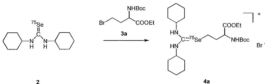
Scheme 2. Formation of the [ 75 Se]selenouronium bromide 4a starting from 1,3-dicyclohexyl[ 75 Se]selenourea 2 and ethyl N-tert-butoxycarbonyl-2-amino-4-bromobutyrate 3a
