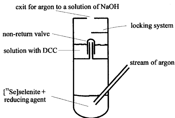
Figure 1. Sketch of apparatus for the synthesis and reaction of [^{75}\text{Se}]\text{H}_2\text{Se}
