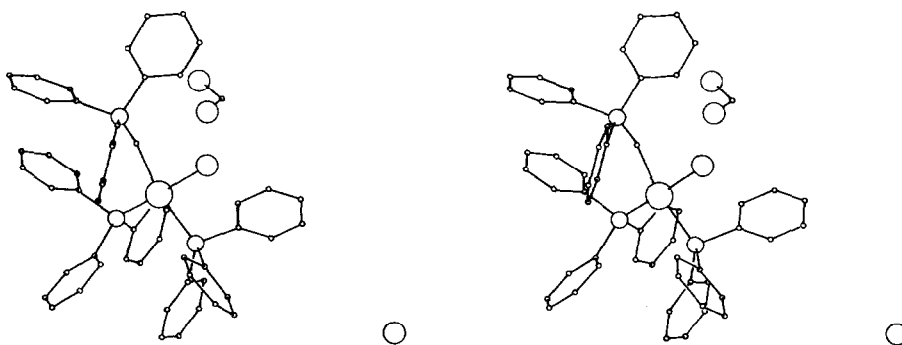
Fig. 2. A stereoview of the structure of \text{cis-}[\text{Pt}(\text{CH}_2\text{PPh}_3)\text{I}(\text{PPh}_3)_2][\text{I}] .
