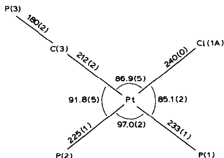
Fig. 3. The coordination about the platinum in \text{cis-}[\text{Pt}(\text{CH}_2\text{PPh}_3)\text{Cl}(\text{PPh}_3)_2][\text{I}] showing bond distances (pm), bond angles ( ^\circ ) and atomic labelling.
