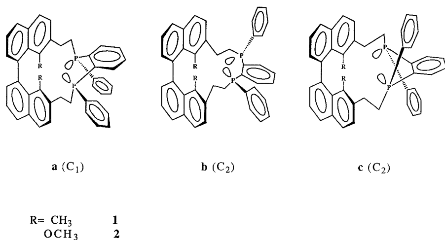
Fig. 1. Diastereomers of compounds 1 and 2
