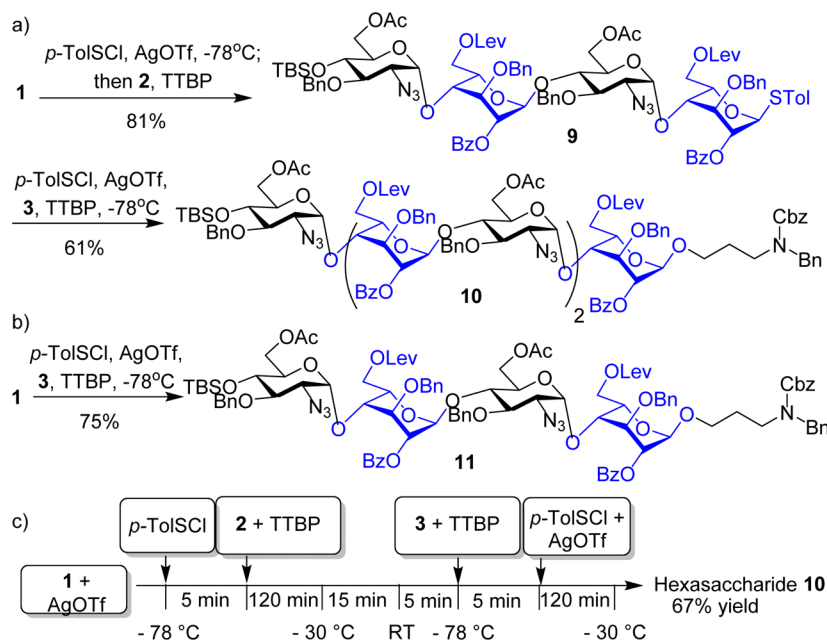
Scheme 2. Synthesis of Heparan Sulfate Backbones 10 and 11
