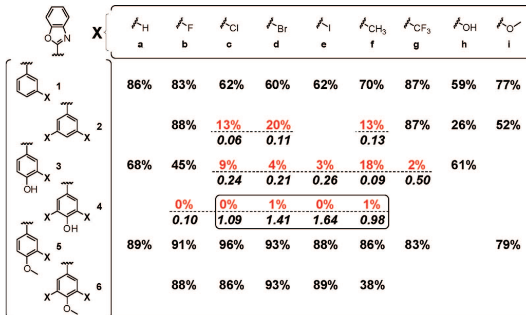
Figure 3. Inhibition of TTR aggregation and stoichiometry of benzoxazole bound to TTR in human blood plasma. Percent (%) values represent the extent of in vitro WT-TTR fibril formation in the presence of inhibitor (7.2 \mu M inhibitor, 3.6 \mu M TTR, pH 4.4, 37 ^{\circ} C, 72 h) relative to aggregation in the absence of inhibitor (100%), with the best values shown in red (<20% aggregation; errors are typically less than \pm 5 percentage points). The average stoichiometries of the most potent aggregation inhibitors bound to TTR in human blood plasma ex vivo are shown in italics (10.8 \mu M inhibitor, 1.8–5.4 \mu M TTR; maximum binding stoichiometry 2) with those exhibiting exceptional binding selectivity to TTR boxed (errors are typically less than \pm 0.1 ).
