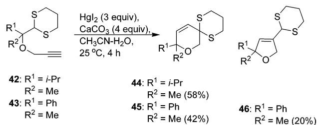
Scheme 5. \text{HgI}_2 Mediated Cyclization of Alkynedithioacetals
