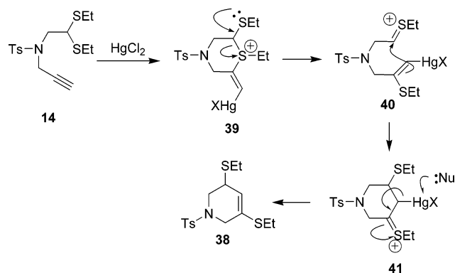
Scheme 4. Tentative Mechanism for the Formation of 38
