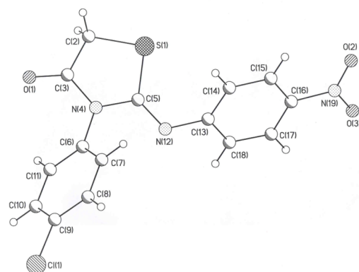
Figure 3. Crystal structure of compound 3d .
