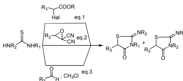
Scheme 1. The reported routes to the synthesis of Iminothiazolidinone derivatives
