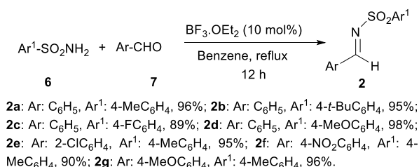
Scheme 2. Synthesis of N -sulfonyl aldimines
