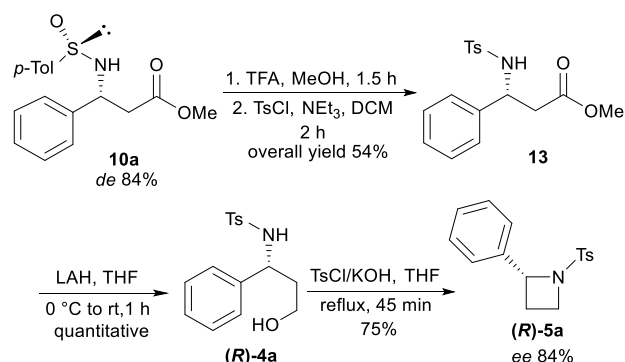
Scheme 5. Synthesis of chiral 2-Aryl- N -tosylazetidine from chiral β-amino ester
