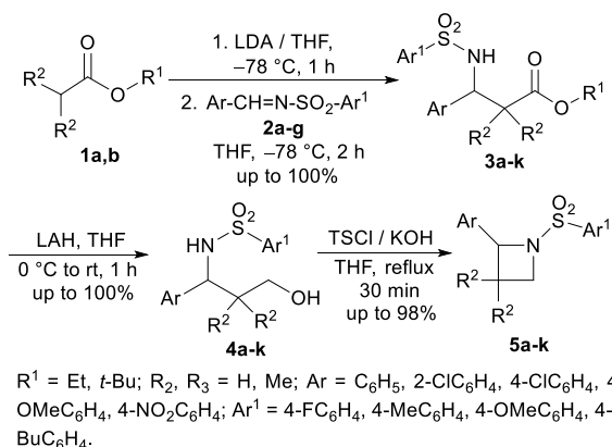
Scheme 3. Synthesis of 2-aryl- N -sulfonylazetidines
