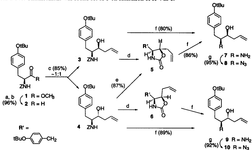
Scheme 1. a) \text{NaBH}_4 , THF/MeOH (20:1), -10\text{ }^\circ\text{C} \rightarrow \text{room temp.} , 16 h; b) Dess-Martin periodinane, \text{CH}_2\text{Cl}_2 , room temp., 1 h; c) Allyl bromide, Zn, THF/aq. \text{NH}_4\text{Cl} (1:5), 0\text{ }^\circ\text{C} , 1.5 h; d) aq. 7.5 M KOH/MeOH/THF (1:2:4), room temp., 5 h; e) \text{MsCl} , \text{NEt}_3 , \text{CH}_2\text{Cl}_2 , 0\text{ }^\circ\text{C} , 2 h then 1,2-dichloroethane, reflux, 24 h; f) aq. 1 M KOH/EtOH (1:1), reflux, 5 h; g) \text{TfN}_3 , DMAP, \text{CuSO}_4 (cat.), \text{CH}_2\text{Cl}_2 , room temp., 2 h.
