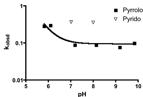
FIGURE 2. pH–rate profile for quinone methide formation from the reduced pyridindole ( 3aH 2 ) and the pyrroloindole ( 3bH 2 ).
