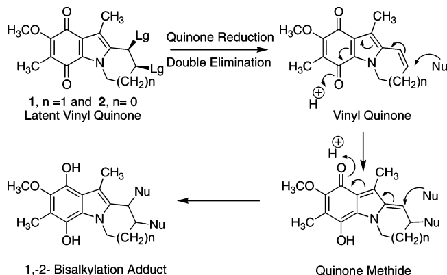
CHART 1. Reductive Activation and Double Leaving Group Elimination
