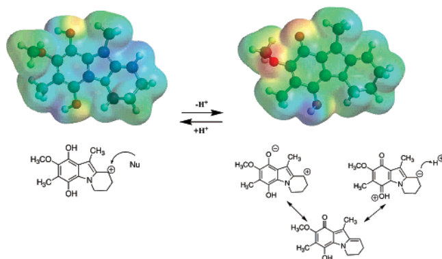
FIGURE 5. Potential density maps for the O-protonated pyridoindole quinone methide and the corresponding neutral species. The charge density color codes are anionic (red), cationic (blue), and neutral (green).
