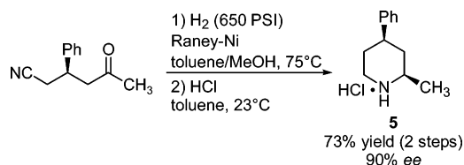
Scheme 4. Preparation of Enantioenriched 2,4- cis -Disubstituted Piperidine
