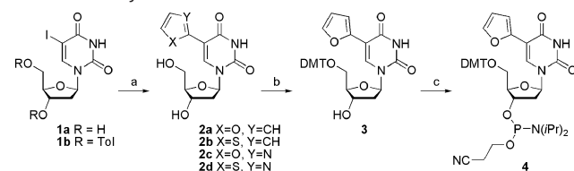
Scheme 1. Synthesis of Nucleosides 2a–d and Amidite 4a
