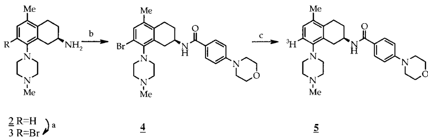
Scheme 1. (a) \text{Br}_2 (b) 4-morpholinobenzoic acid/CDI (c) ^3\text{H}_2/\text{PdO}
