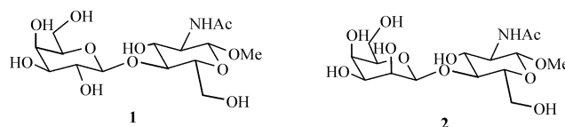
Fig. 1 Compounds 1 and 2 .
