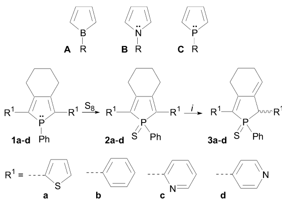
Scheme 1 Conditions: i , 3a : refluxing xylene, Et 2 NH, 1 day; 3b : refluxing xylene, Et 2 NH, 4 h; 3c, d : 40 °C, THF, 2 days. Dotted lines show the connectivity of the R 1 substituents.
