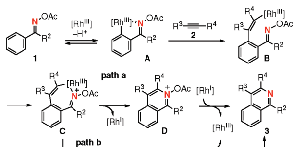
Scheme 2. Proposed Mechanistic Possibility
