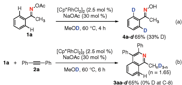
Scheme 1. Investigation of the Reaction Mechanism
