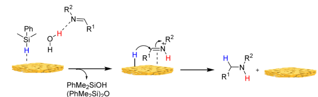
Scheme 3. Plausible Pathway for Imine Reduction
