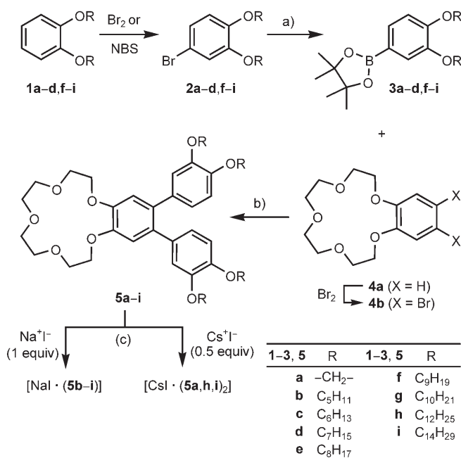
Scheme 1. Preparation of crown ether derivatives 5 : a) BuLi (1.25 equiv), –78°C, B(OMe) 3 (1.25 equiv), –78°C→RT, pinacol (1.25 equiv), AcOH (1.25 equiv), 18 h; b) DME/H 2 O, + 3 (2.2 equiv), K 2 CO 3 , KF (10 equiv each), [Pd(PPh 3 ) 4 ], 95°C, two days; c) + MX, 1–2 h, RT.
