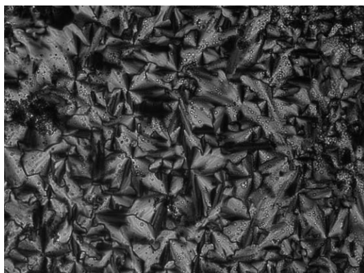
Figure 5. Fan-shaped texture of the complex NaI·5h as seen between crossed polarizers at 139°C upon slow cooling from the isotropic phase (magnification \times 200 ).
