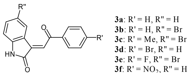
Figure 2. Known biologically active non-glycosylated 3-alkylideneoxindoles
