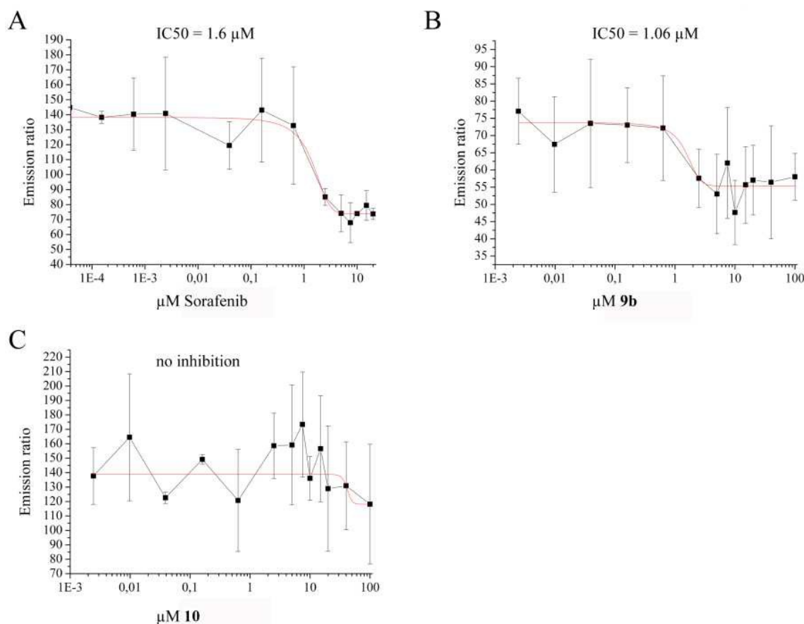
Figure 8. Derivative 9b strongly inhibits JNK2 activity in melanoma cells. Kinase ATP-binding assays were performed with recombinant JNK2 using different concentrations of the positive control inhibitor sorafenib as well as of derivatives 9b and 10 . Experiments were performed three times each in triplicates. \text{IC}_{50} values were calculated after analysis of all experiments. Graphs correspond to the means of one representative experiment.
