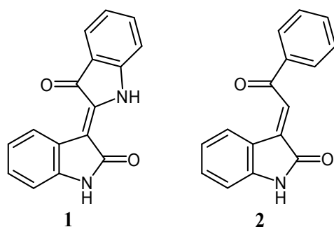
Figure 1. Indirubin ( 1 ) and 3-alkylideneoxindole 2
