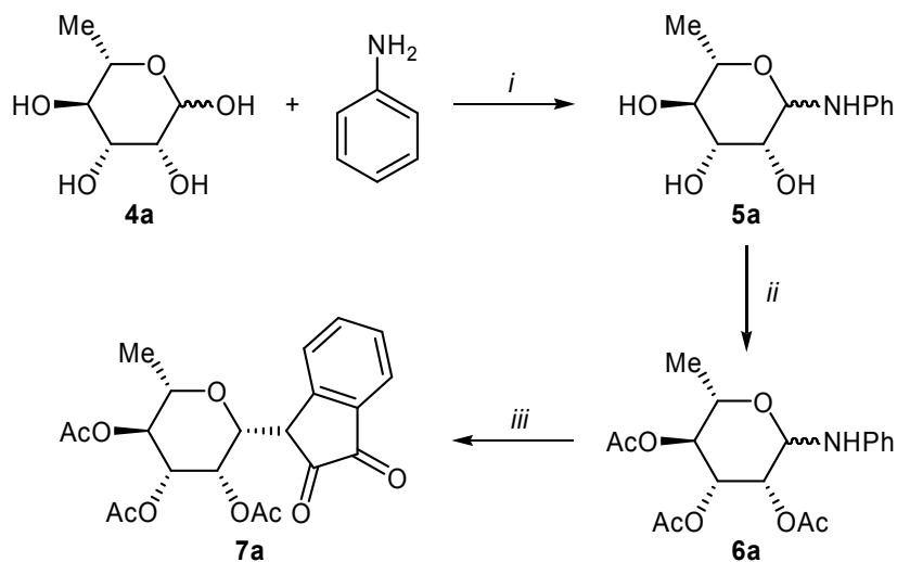
Scheme 1. Synthesis of 1-(2,3,4-tri- O -acetyl-β-L-rhamnopyranosyl)isatin ( 7a ). Reagents and conditions: (i) PhNH 2 , EtOH (abs.), 20°C, 24 h; (ii) Ac 2 O, pyridine, 0 °C, 12 h; (iii) oxalyl chloride (10 equiv.), AlCl 3 (1 equiv.), 55°C, 1.5 h, then chromatographic separation of the anomers.
