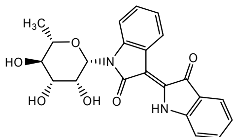
Figure 7. Structure of the N - \beta -L-rhamnopyranosylindirubin 10 used as control substance.
