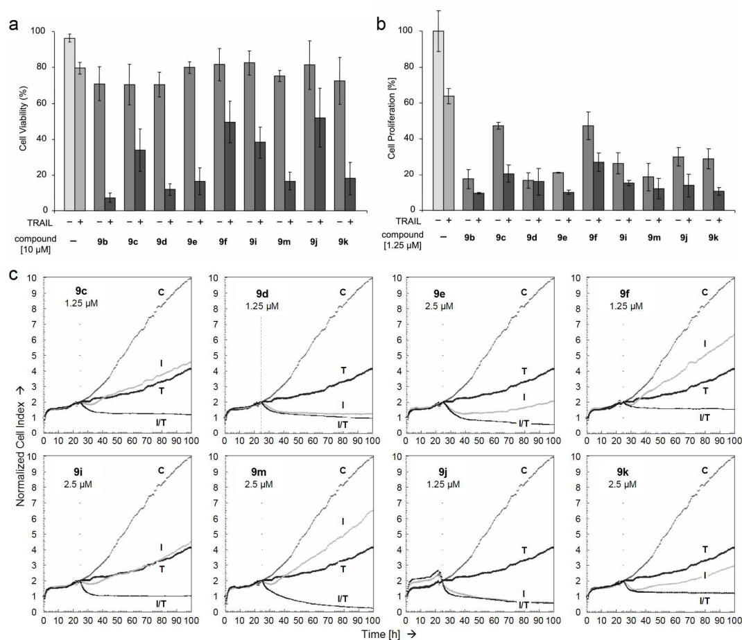
Figure 5. Effects of N -glycosylated 3-(2-oxo-2-arylethylidene)indolin-2-ones on melanoma cells: (a) Cell viability of A-375 cells was determined after 24 h by calcein staining. Cells were treated with TRAIL (20 ng/ml), compounds of the series 9 (10 \mu\text{M} ) or with combinations. (b) Cell proliferation of A-375 cells expressed as percent of non-treated controls was determined after 48 h by WST-1 assay. Cells were treated with 1.25 \mu\text{M} of compounds of series 9 and/or 20 ng/ml TRAIL. (c) Real-time cell analysis (RTCA) of A-375 cells treated with 1.25 \mu\text{M} / 2.5 \mu\text{M} of 9c , 9d , 9e , 9f , 9i , 9m , 9j and 9k +/- 20 ng/ml TRAIL. Seeding density was 1,250 cells per microtiter well. The cell index was normalized at 24 h,
