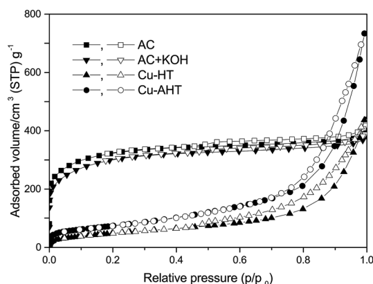
Fig. 1 Adsorption isotherms of nitrogen obtained at -196^\circ\text{C} on parent carbon (AC) and the 30KOH/AC samples (AC + KOH) as well as on copper loaded hydrotalcite precursor calcined at 200^\circ\text{C} (Cu-HT) and 520^\circ\text{C} (Cu-AHT).
