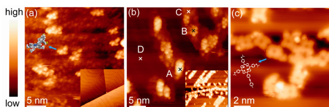
Figure 3. (a) STM image of 1 as prepared via drop-casting on Au(111) (2.8 V, 10 pA, 25 \times 25 nm 2 ). The inset shows the Au(111) surface before deposition (2.5 V, 100 pA, 80 \times 80 nm 2 ). (b) STM image upon annealing at \sim 310 °C for \sim 1 h (2.8 V, 20 pA, 30 \times 30 nm 2 ). The inset is an image of a larger area (2.8 V, 5 pA, 75 \times 75 nm 2 ) with a discernible herringbone feature on the bare Au surface. (c) High-resolution image upon further annealing at \sim 400 °C for \sim 1 h (2.5 V, 10 pA, 12 \times 12 nm 2 ).
