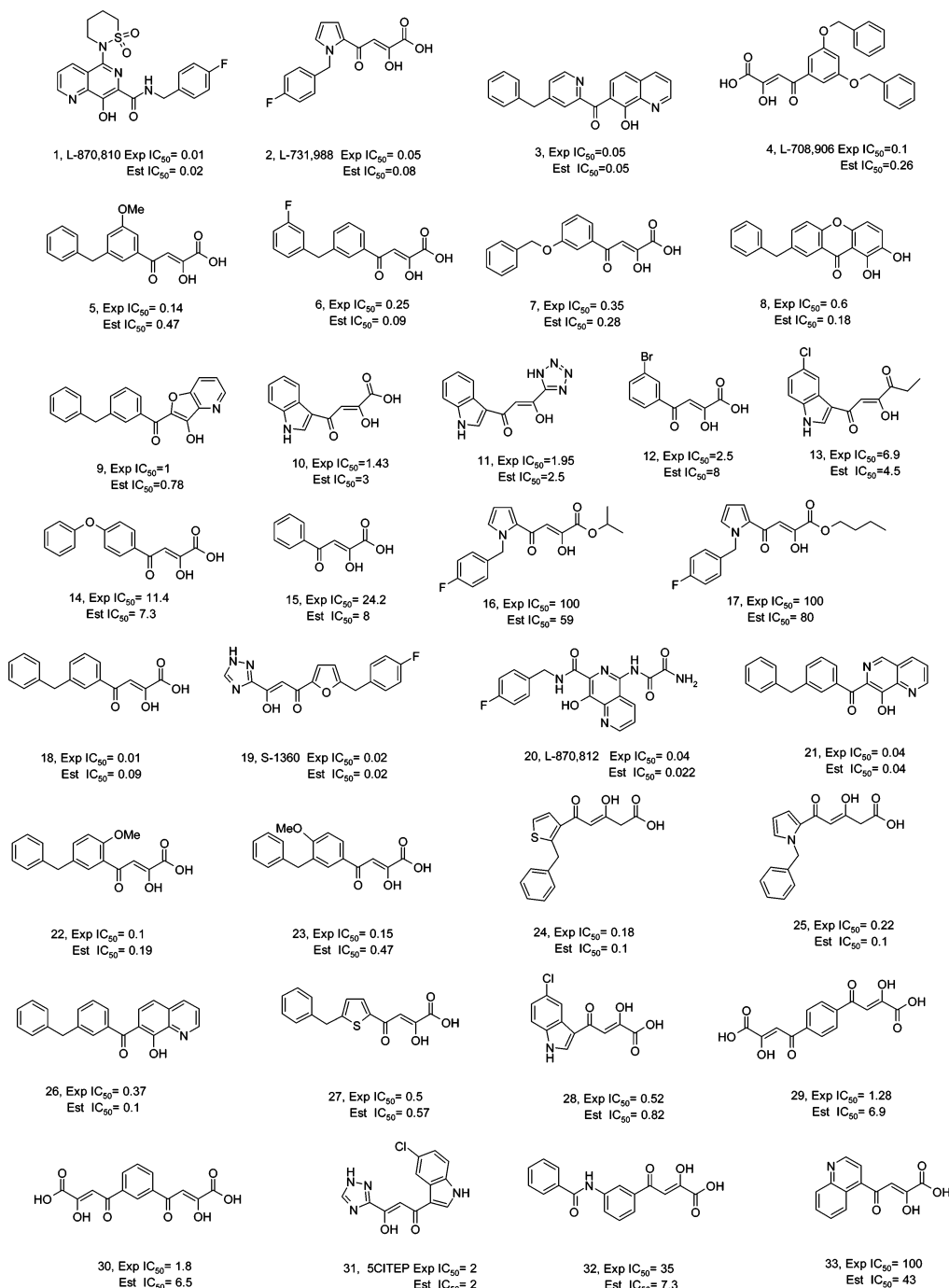
Figure 1. Chemical structures of the 33 data set molecules (TS, 1–17 and PS, 18–33) with their experimental (exp IC 50 ) and estimated (est IC 50 ) IN strand transfer inhibitory activities, both expressed in μM.
