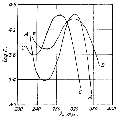
A, 5-Benzylidenehydantoin in alcohol. B, 5-Benzylidene-3-methylhydantoin in N /100-alcoholic NaOEt. C, Cinnamoylurea.
