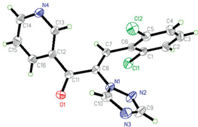
FIGURE 1 Molecular structure and crystallographic numbering for compound 4g . Selected bond lengths (Å): Cl (1)–C (1) 1.7292 (17); Cl (2)–C (5) 1.7373 (17); O (1)–C (11) 1.212 (2); N (1)–C (10) 1.339 (2); N (1)–N (2) 1.3608 (19); N (1)–C (8) 1.418 (2); N (3)–C (10) 1.306 (2); N (4)–C (13) 1.330 (2); C (5)–C (6) 1.392 (2); C (6)–C (7) 1.475 (2); C (7)–C (8) 1.328 (2). Selected angles (°): O (1)–C (11)–C (8) 120.44 (15); O (1)–C (11)–C (12) 120.06 (15); C (12)–C (11)–C (8) 119.49 (14); C (7)–C (8)–N (1) 121.81 (15); C (7)–C (8)–C (11) 123.08 (15); N (1)–C (8)–C (11) 114.82 (13); C (6)–C (7)–C (8) 126.28 (15); C (10)–N (1)–N (2) 108.82 (14); C (10)–N (1)–C (8) 129.33 (14); N (2)–N (1)–C (8) 121.83 (13); C (10)–N (3)–C (9) 101.71 (15); C (13)–N (4)–C (14) 116.31 (16); N (4)–C (14)–C (15) 124.48 (18).
