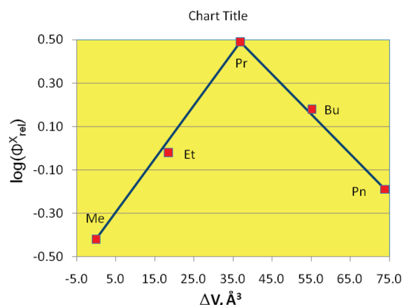
Figure 3. Effect of the N -alkyl substituent on \log(\Phi^X_{rel}) .
