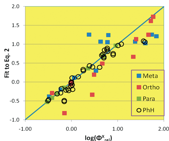
Figure 2. Fit of eq 2 to the experimental data.
