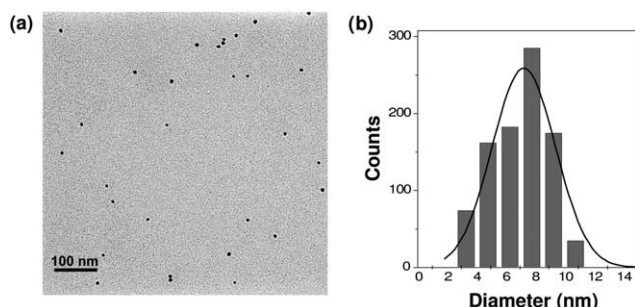
Fig. 1 (a) Selected TEM image of Pd(0)-NPs dispersed in (BCN)MI·NTf 2 and (b) the histogram showing the particle size distribution of Pd(0)-NPs dispersed in (BCN)MI·NTf 2 . The particles display an irregular shape with a monomodal particle size distribution of 7.3 ± 2.2 nm.
