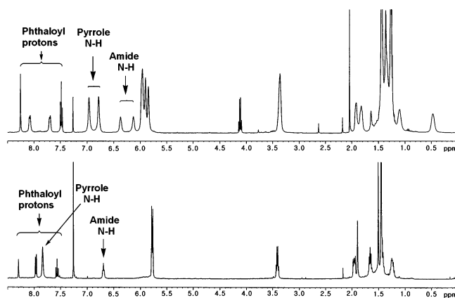
FIGURE 1. Typical proton NMR spectra at cis-strapped ( 13 ) (bottom trace) and trans-strapped ( 15 ) (top trace) calix[4]-pyrroles in \text{CDCl}_3 at 25 °C.
