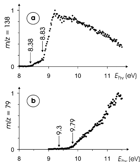
Figure 2. Single-ion monitoring of (a) m/z = 138 (parent ion) and (b) m/z = 79 ( C_6H_7^+ ) as a function of photon energy (eV). The appearance energies referred to in the text are derived from extrapolation of the linear part of the thresholds to the baseline without applying any further corrections.
