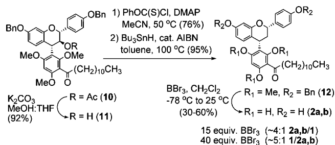
Scheme 3. Completion of (–)-(2a,b) Synthesis
