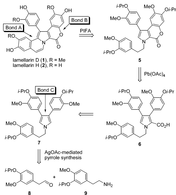
Scheme 1. Retrosynthesis of Lamellarins D and H
