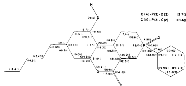
Figure 3. Bond angles are given in degrees. Estimated standard deviations for the last digit are given in parentheses.
