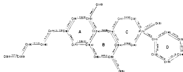
Figure 2. Bond distances as given in Å. Estimated standard deviations for the last digit are given in parentheses.
