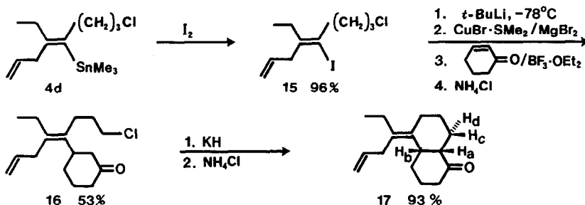
Scheme III
