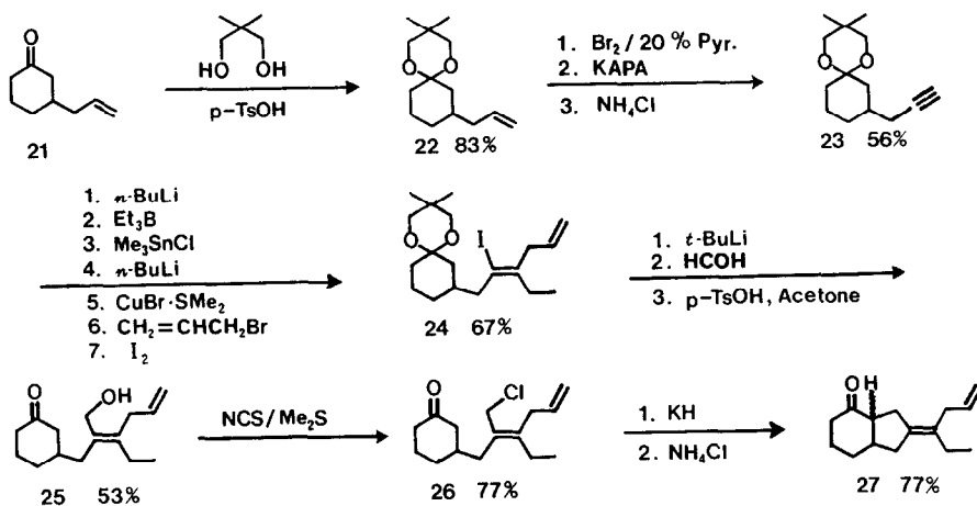
Scheme IV
