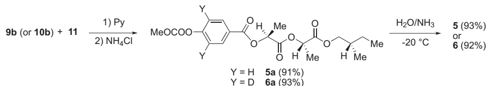
Scheme 4. Preparation of (3 S ,7 S ,10 S ) 10-(4'-hydroxy)benzoyloxy-3,7-dimethyl-5,8-dioxo-6,9-undecandione ( 5 ) and the corresponding 3',5'-dideutero derivative ( 6 ).
