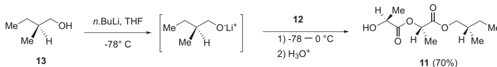
Scheme 3. Preparation of (3 S ,7 S ,10 S ) 10-hydroxy-3,7-dimethyl-5,8-dioxo-6,9-undecandione ( 11 ).
