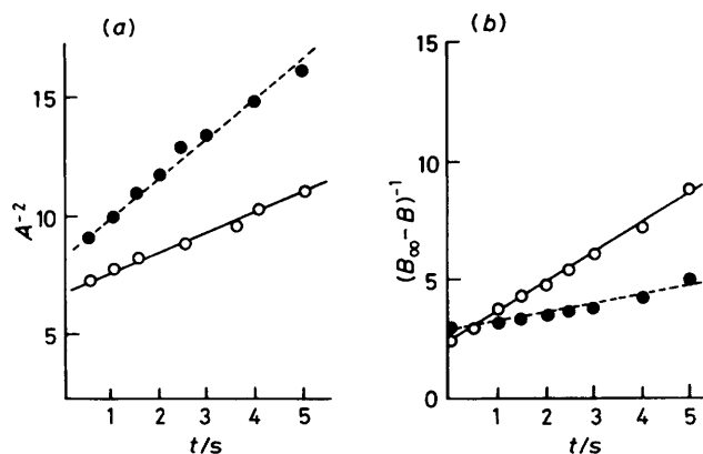
Figure 5. Plots of (a) A^{-2} vs. t and (b) (B_{\infty} - B)^{-1} vs. t for the changes of transients A (780 nm) and B (630 nm) with (—○—) and without (—●—) 0.5 \text{ mol dm}^{-3} cyclohexene. Optical pathlength of the cell is 96 mm
