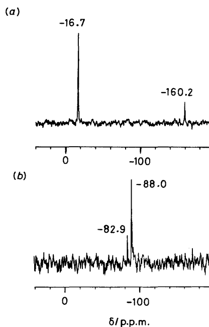
Figure 8. ^{183}\text{W} N.m.r. spectra (20.8 MHz) of [\text{NBu}_4]_4[\text{W}_{10}\text{O}_{32}] in \text{CD}_3\text{CN} -cyclohexene before (a) and after (b) long-term photolysis
