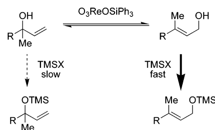
FIGURE 4. Using silylation to control product selectivity.
