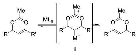
FIGURE 1. Mechanism of “cyclization-induced” rearrangements.
