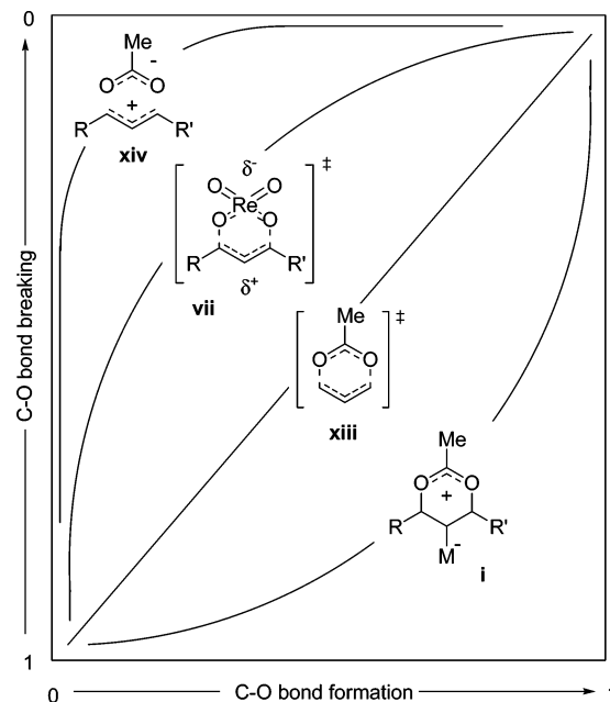
FIGURE 6. Comparison of mechanistically distinct [3,3]-rearrangements.
