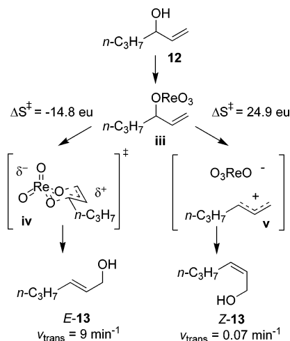
FIGURE 3. Proposed mechanism for \text{O}_3\text{ReOSiPh}_3 -catalyzed isomerizations.
