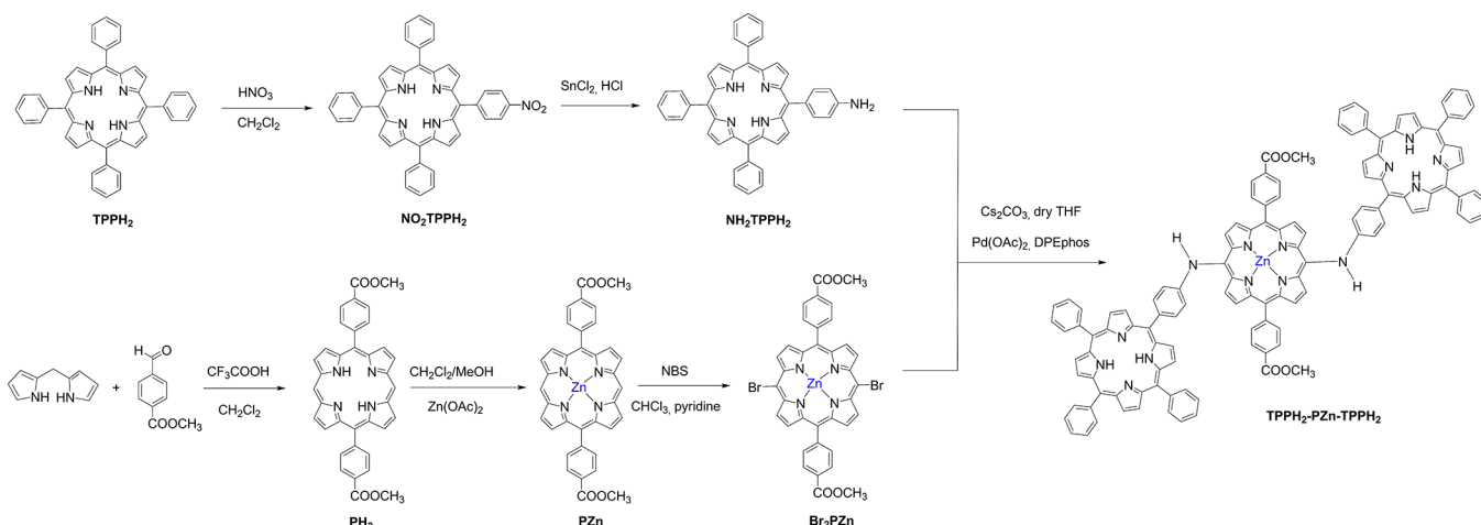
Scheme 1. Synthesis of Trimer \text{TPPH}_2\text{-PZn-TPPH}_2
