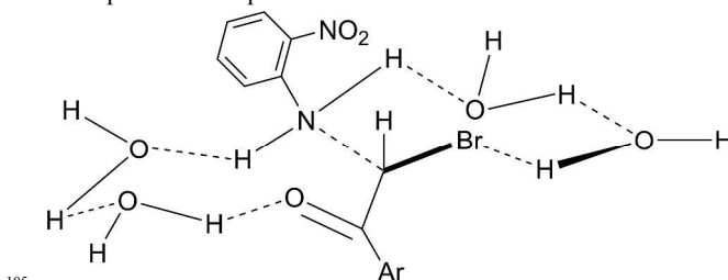
Scheme 4. The envisaged role of water in promoting N -arylmethylation of 1 with 2 to form 3.
