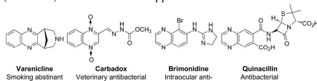
Scheme 1. A few quinoxaline-based drugs.
