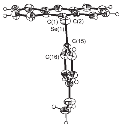
Figure 1. Structure of 1c (S-A) (thermal ellipsoids are shown at 40% probability levels). Selected bond lengths (Å), angles (°), and torsional angles (°): Se(1)–C(1) 1.931(5), Se(1)–C(15) 1.925(5), C(1)–Se(1)–C(15) 99.4(2), C(2)–C(1)–Se(1)–C(15) 95.6(4), C(1)–Se(1)–C(15)–C(16) 174.8(4).
