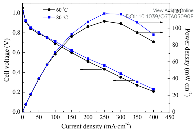
Fig. 9 Fuel cell performance of MEA using the PES-6-QA membrane at 60 and 80 °C.
