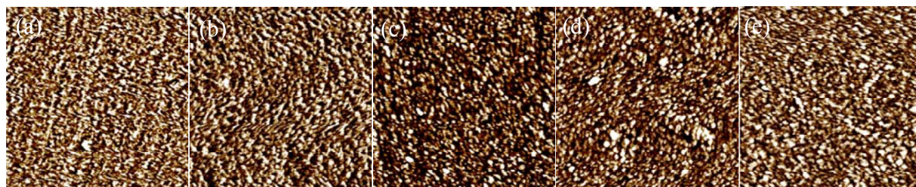
Fig. 1 AFM phase images of (a) PES-3-QA, (b) PES-4-QA, (c) PES-6-QA, (d) PES-8-QA and (e) PES-12-QA. Scan box: 500 nm×500 nm
