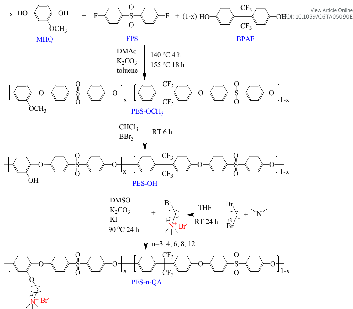
Scheme 1 Synthetic route of Br-n-QA, PES-OCH 3 , PES-OH and PES-n-QA.
