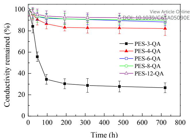
Fig. 7 Hydroxide conductivity changes of the PES- n -QA ( n =3, 4, 6, 8, 12) membranes in a 1 M KOH solution at 60 °C.
