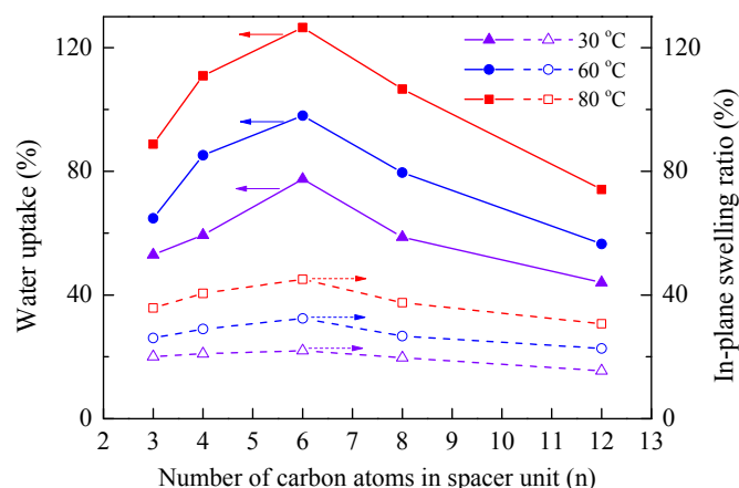
Fig. 2 Water uptake and swelling ratio as a function of flexible spacer length for PES- n -QA membranes at 30, 60 and 80 °C.
