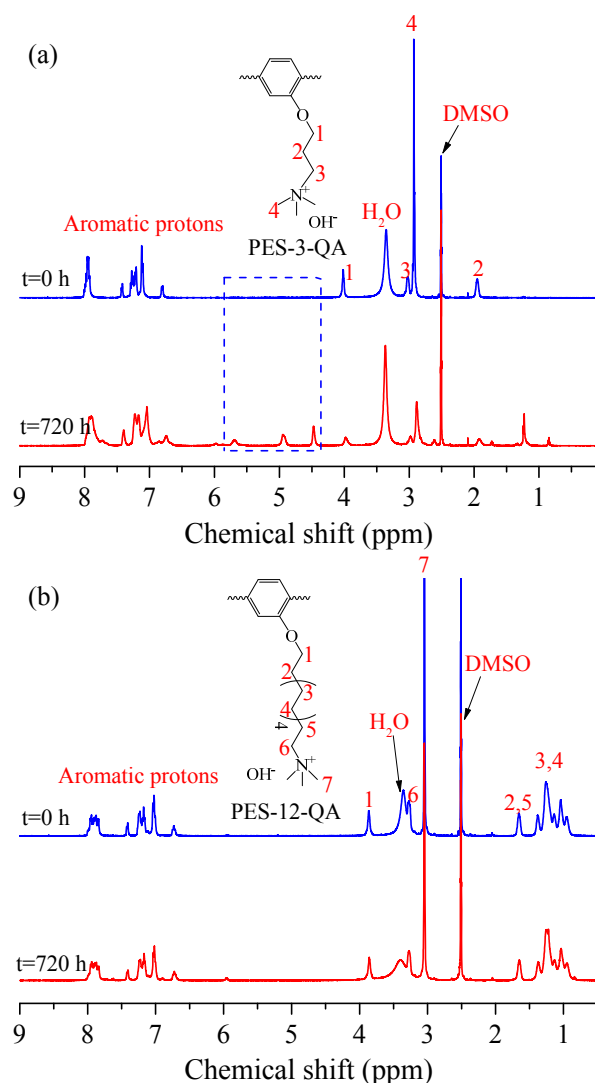
Fig. 8 ^1\text{H} NMR spectra of (a) PES-3-QA and (b) PES-12-QA stored in a 1 M aqueous KOH solution at 60 °C for 0 and 720 h, respectively.
