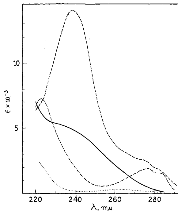
Fig. 1.—Absorption spectra in C_2H_5OH of: CH_3-CO-O-C_6H_5 .....; CH_3-CO-S-C_6H_5 ——; CH_3-CO-O-C_6H_4-OCH_3 -----; CH_3-CO-S-C_6H_4-OCH_3 — · — · —.
