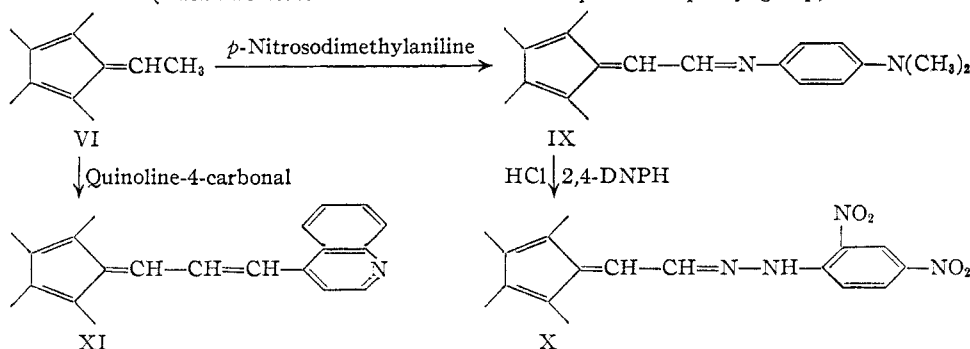
CHART II THE CHEMISTRY OF 6-METHYL-1,2,3,4-TETRAPHENYLFULVENE (Each line attached to a central nucleus represents a phenyl group)
