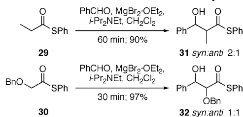
Scheme 2. MgBr 2 ·OEt 2 -Promoted Direct Aldol Reaction of α-Substituted Thioesters with Benzaldehyde a
